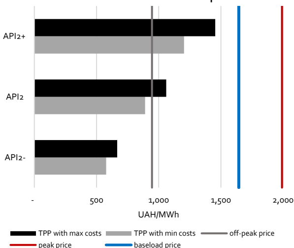
Figure 13. Marginal costs of coal TPP in Ukraine under different coal prices
